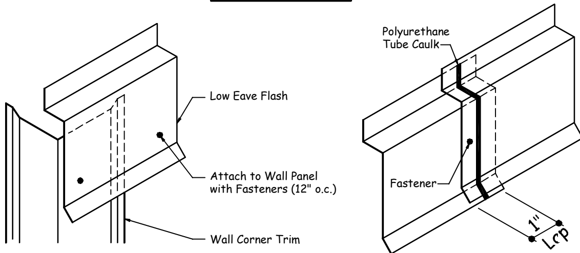
WALL SECTION
