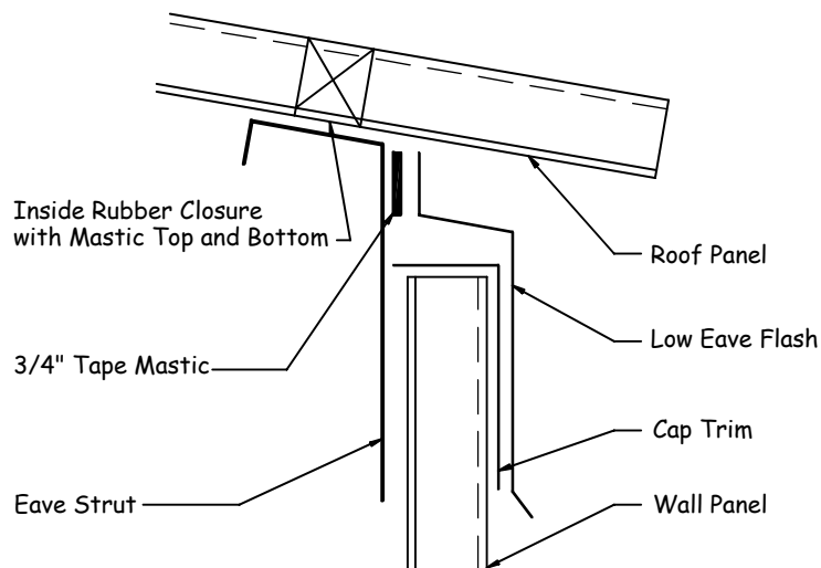
WALL SECTION
